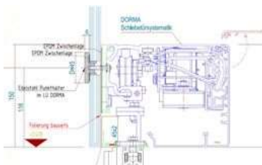
dokaIA Manet
