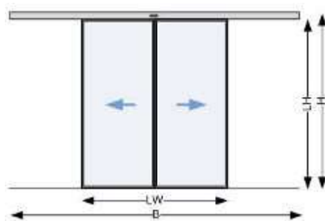
dokaIA ST 5
