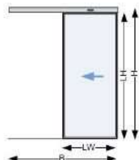
dokaIA ST 1
